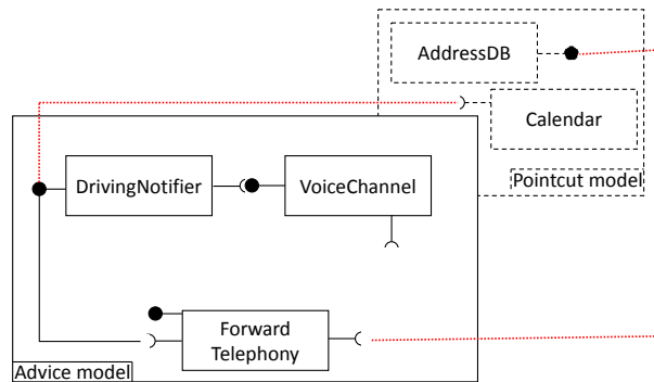
Fig. 1. An Aspect Model
