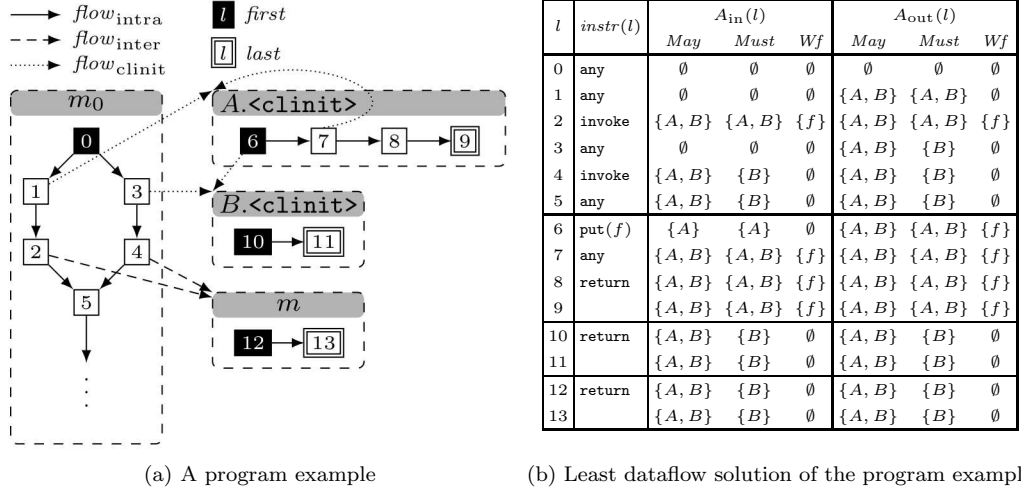
Fig. 7. Program and analysis example
