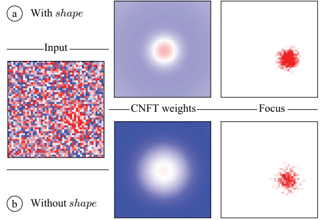
Fig. 5. Qualitative difference in the optimal solution and CNFT lateral kernel relatively to the use of shape in the fitness evaluation. Although the stimulus is hard to distinguish on the noisy input (of standard deviation 1.0), both sets of optimal parameters found by the GA accurately track it. The GA however converge to different parameter values due to the tradeoff between fast convergence ( conv ) and resilience/lack of distortions ( shape ). (a) The top row screenshots show the CNFT weights and focus field obtained when integrating the shape variable. The excitatory core produces a well-formed bubble by reinforcing its spatial coherence. (b) The bottom row shows the same elements without the use of shape in the fitness.
