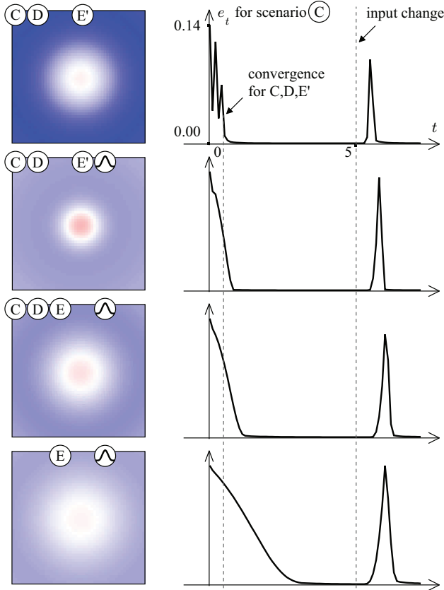
Fig. 4. Comparison of the lateral connection kernels and error dynamics on scenario [C]. This scenario is the only one without a random component in it, allowing reproducible deterministic dynamics without using statistics over a large number of trials. Each row represents the results on a different set of scenarios and variables used to evolve the parameter vector population. When using the shape variable and scenario [E], the model loses in reactivity but gains in smoothness and stability.
