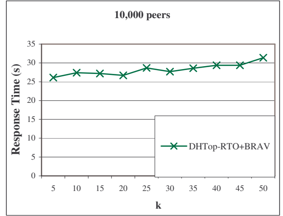
Figure 5. Response time vs. k
