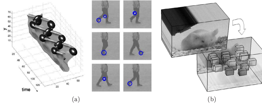
Figure 5: Local posture representations: (a) Space-time interest points in [86] are computed at points of high spatiotemporal variation ("spatiotemporal corners"). (b) Spatio-temporal features in [32] are designed to be more responsive than the former space-time interest points. Awaiting publisher permission
