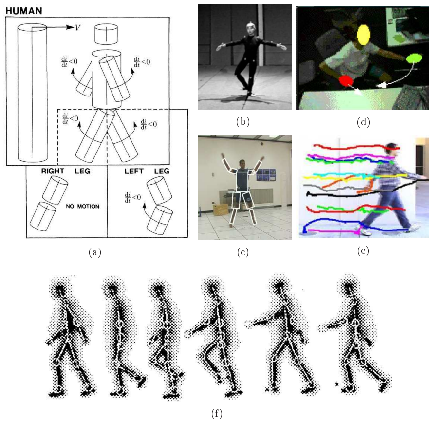
Figure 3: Model based posture representations: (a) hierarchical 3D model based on cylindrical primitives [103]; (b) ballet dancer with markers attached to body [22]; (c) body model based on rectangular patches [133]; (d) blob model [19]; (e) 2D marker trajectories [200]; (f) stick figure [58]. Awaiting publisher permission
