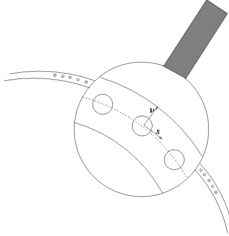
Figure 2: the scaled variables S and \mathcal{V}
