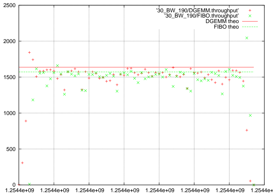
Figure 8: Throughputs obtained when modeling with 186.7 Mb.s^{-1}
