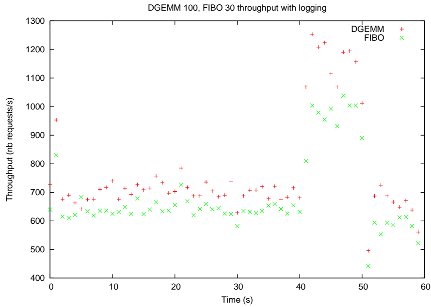
Figure 58: Throughput for dgemm 100, Fibonacci 30. With logging on.
