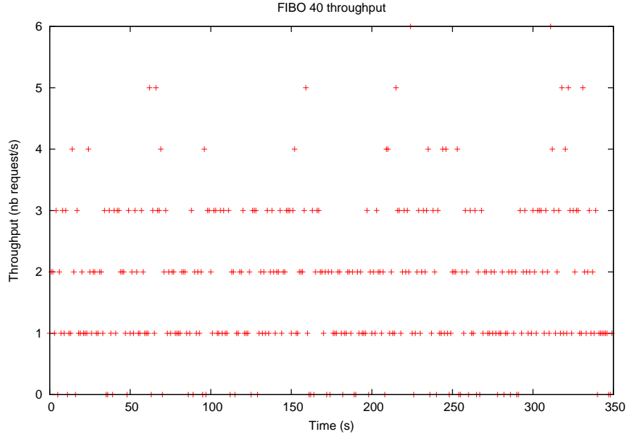
Figure 18: FIBO 40 throughput
