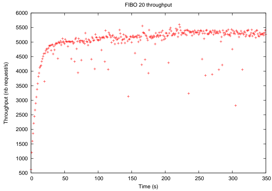
Figure 16: FIBO 20 throughput
