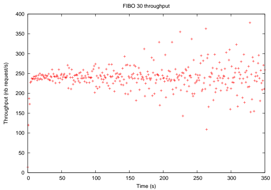
Figure 17: FIBO 30 throughput
