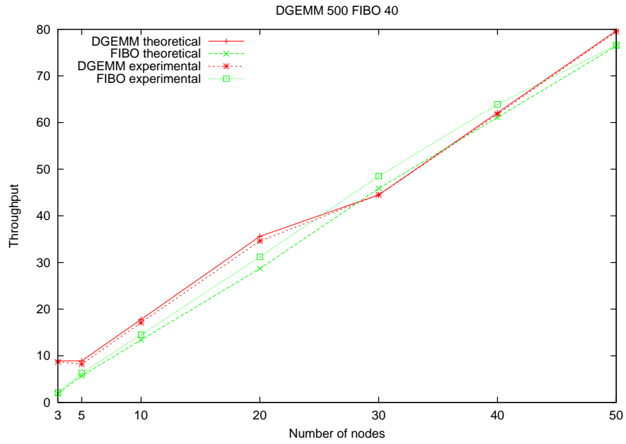
Figure 50: Comparison theoretical/experimental results, for dgemm 500 Fibonacci 40.
