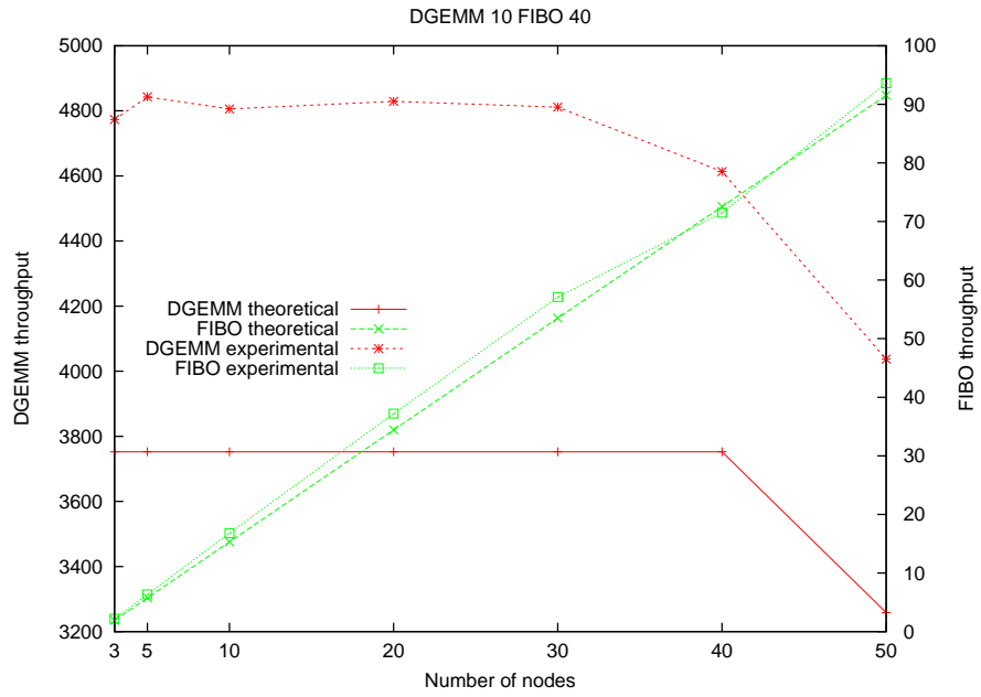
Figure 34: Comparison theoretical/experimental results, for dgemm 10 Fibonacci 40.
