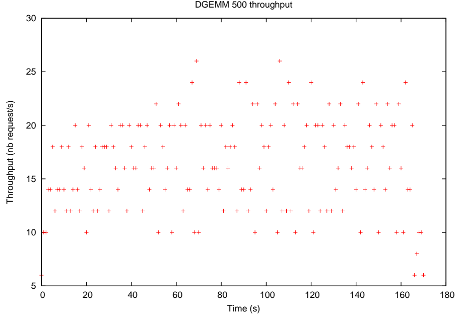
Figure 15: dgemm 500 throughput
