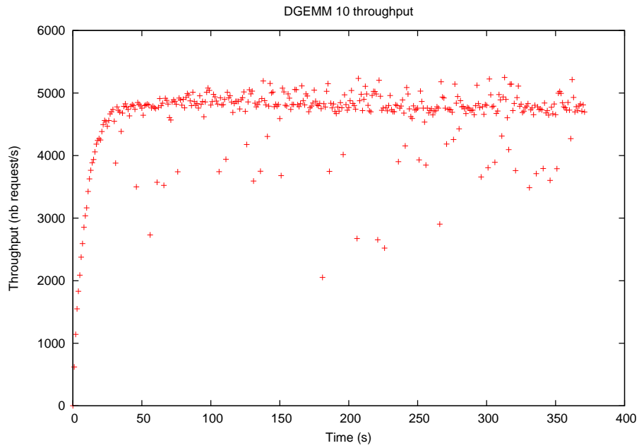
Figure 13: dgemm 10 throughput
