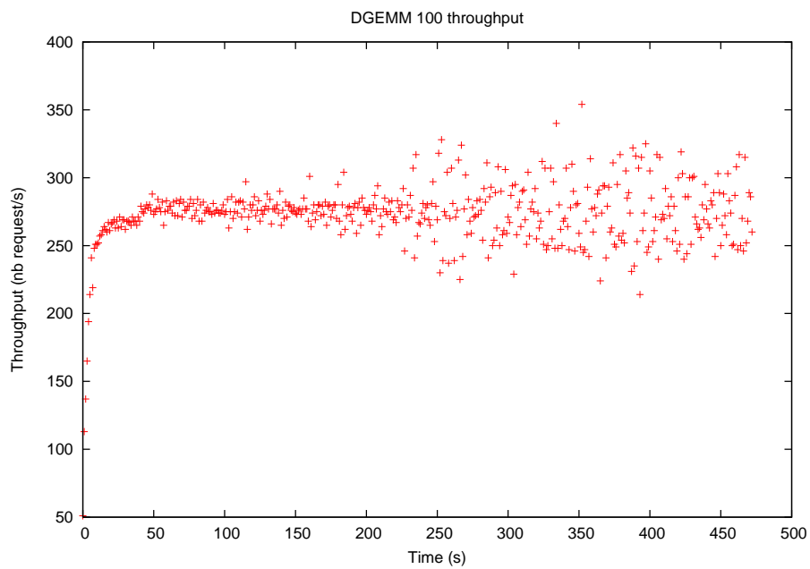
Figure 14: dgemm 100 throughput
