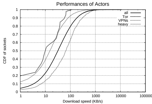
Figure 16: Performance of peers. all is for the 3M of peers for which we performed a download measure.
