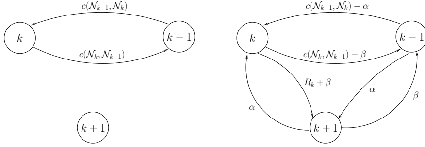
Figure 3. Modifications when adding \mathcal{N}_k + 1 .
