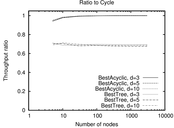
(a) Comparison of algorithms to CYCLICRA
