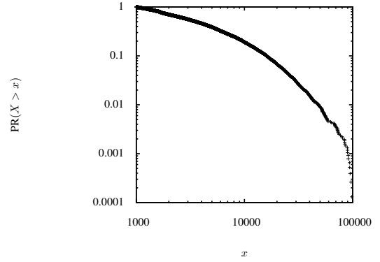
Figure 4. Complementary CDF of the distribution used to generate bandwidth values.
