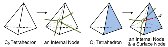
Figure 5: Construction QuadGraph from tetrahedron mesh. Left: a C_0 tetrahedron is converted to an inner node (Green). Right: a C_1 tetrahedron is converted to an inner node (Green) and a surface node (Red).
