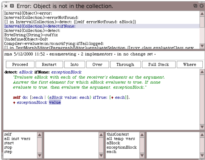
Figure 6.25: The debugger.
