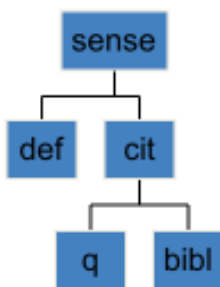
190 Figure 3: tree representation of the above XML fragment
