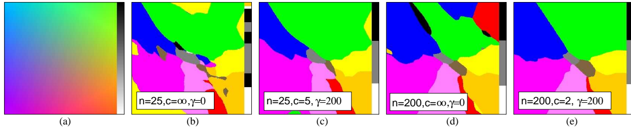
Fig. 6. (a) A challenging synthetic image: the highly saturated RGB values at the border rarely occur in natural images. (b-e) results obtained with different settings for c , \gamma and n the number of train images per color name. The figure demonstrates that our method, images (c) and (e), improves results.
