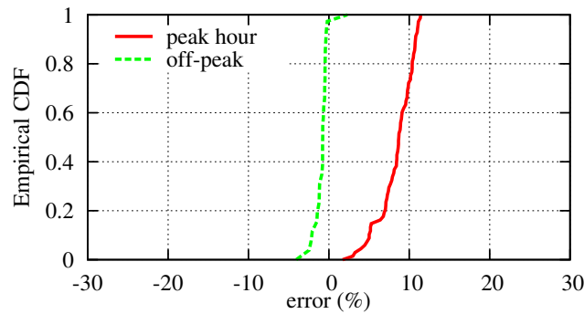
Figure 12: Empirical CDF of the error between the RTT measured at the source and estimated (Internet experiments).
