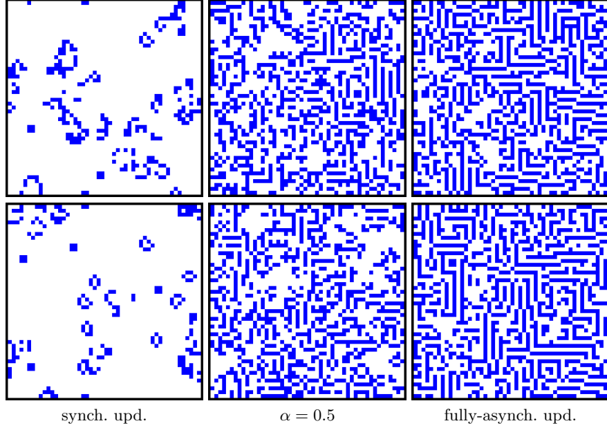
Fig. 1. Snapshots of configurations obtained with 3 updating schemes: synchronous (left), \alpha -asynchronpous (middle), fully asynchronous (right). Configurations are taken at time \tau = 100 (top) and \tau = 200 (bottom).
