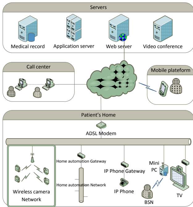
Fig. 2. Hardware architecture
