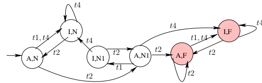
Fig. 9. \text{OBS}(G_\Omega) for \Sigma_o = \{t_1, t_2, t_4\}
