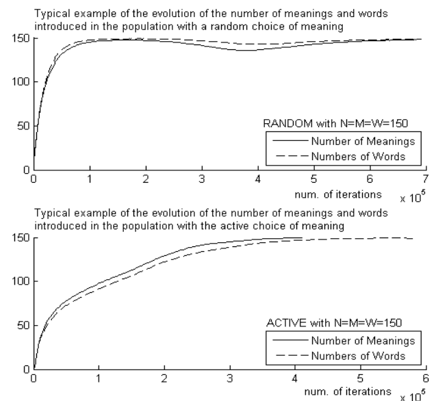
Figure 2 With the active choice of meaning, the growth of the number of meanings and words is dynamically controlled.
