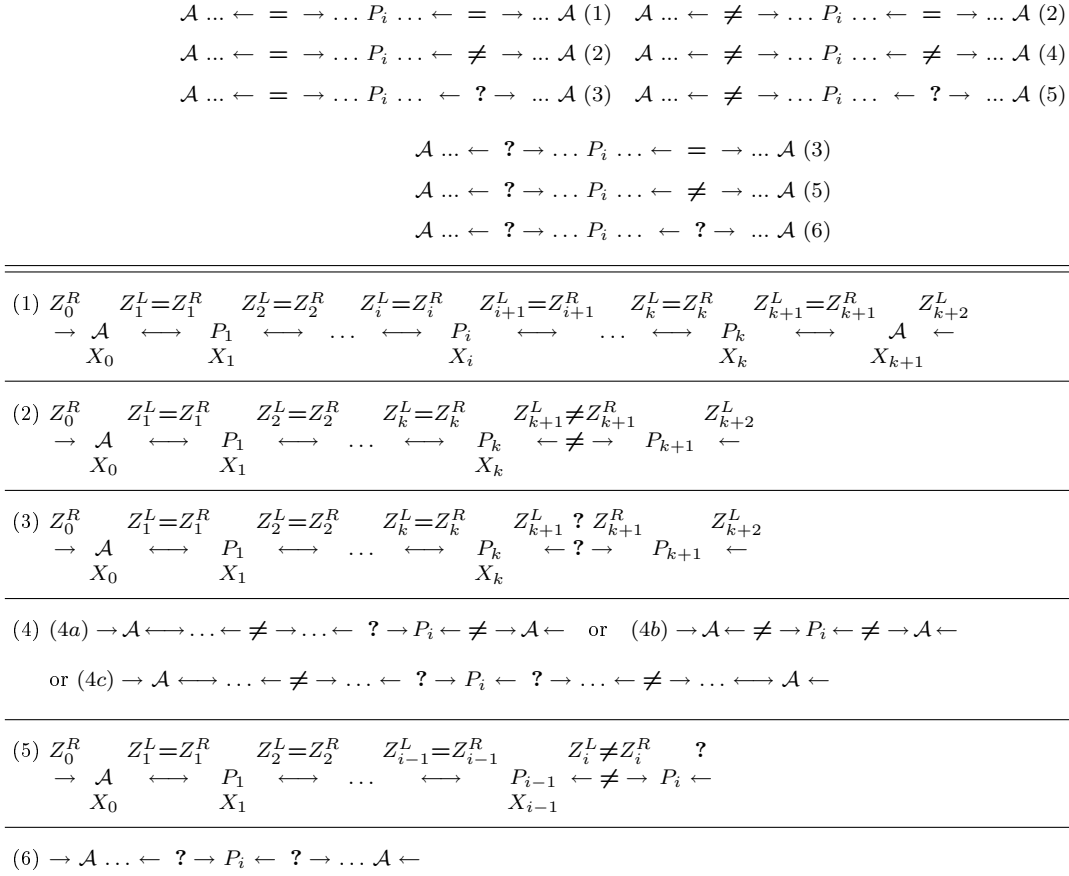
Fig. 6. The different cases of connected components
