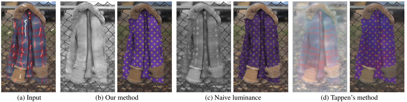
Figure 12: Our approach (b) produces illumination maps that are more accurate than luminance (c) for re-texturing textured objects. On this highly textured image, the automatic classifier of Tappen et al.[2005] cannot decompose reflectance and illumination properly (d), which impacts the result of the manipulation.
