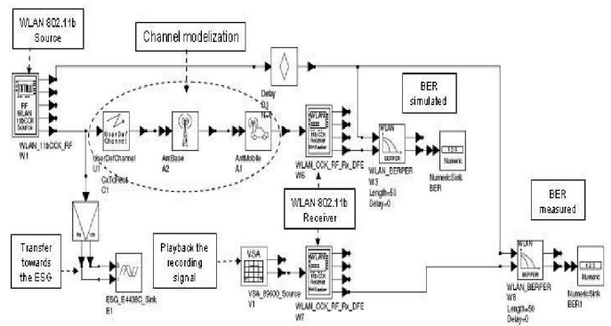
Fig. 2. Example of a schematic design for 802.11b BER evaluation
