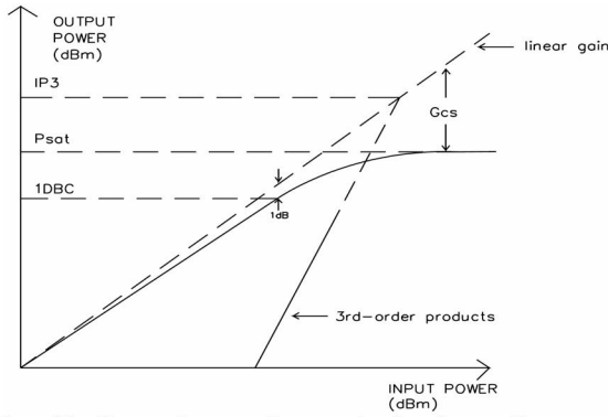
Fig. 8 Nonlinear element characterization for nonlinear models
