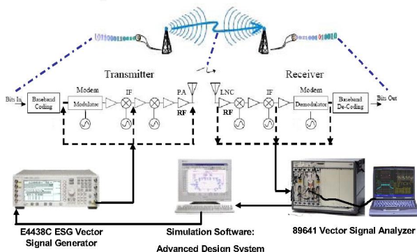
Fig. 1. The platform structure for a 1x1 transmission
