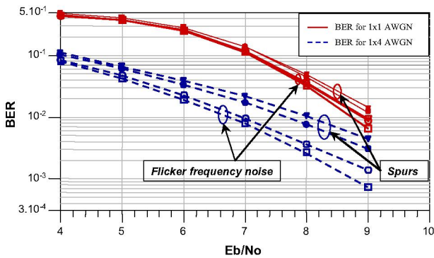
Fig. 10 Influence of phase noise (-30dB/dec) and PLL spurious on BER performances.
