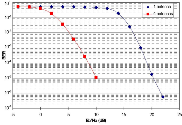
Fig. 4. BER vs. Eb/No in multipath channel
