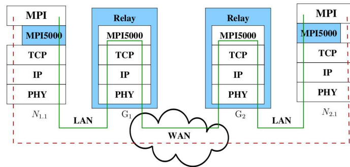
Figure 6: Architecture de MPI5000
