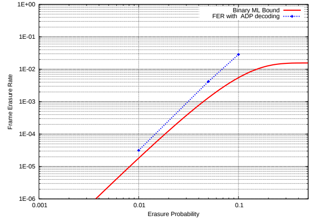
Fig. 3. Comparaision of the simulated ADP decoding performance with the Maximum Likelihood Bound for the Reed Solomon (7,5).
