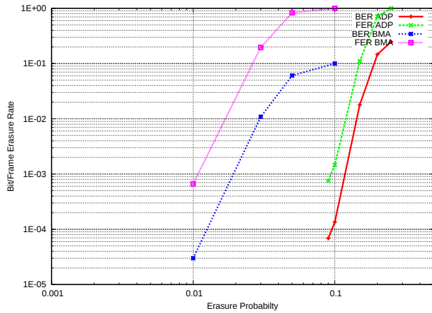
Fig. 4. Performance of the Reed Solomon Code (31,25) over the BEC.
