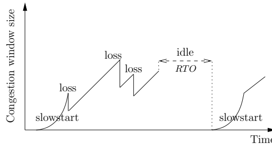
Figure 2: Evolution of TCP congestion window
