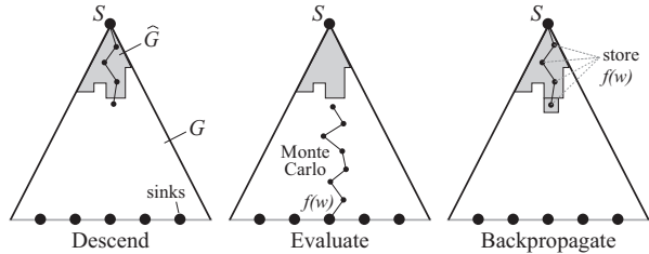
Figure 2. Visualization of the three main steps in TAG. Note that \hat{G} (shaded area) and G are not trees (e.g., see Figure 1).
