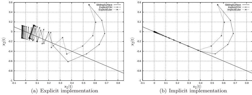
Figure 7: Comparison of Euler and ZOH discretizations of ECB-SMC system, a_1 = -2 , a_2 = 2 , c_1 = 1 and h = 0.3 . x_0 = [0.55, 0, 55]^T State x_1(t) versus x_2(t) .
