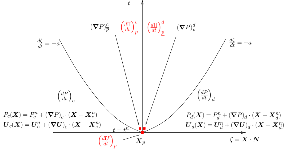
Figure 10: Structure of the Generalized Riemann problem at point p in the direction of the unit normal \mathbf{N} . Note that \zeta = \mathbf{X} \cdot \mathbf{N} is the variable in the direction of \mathbf{N} .
