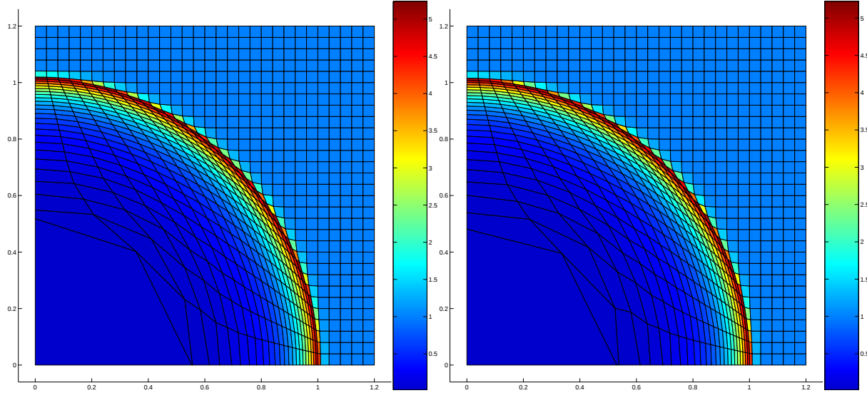
Figure 19: Density map for the Sedov problem on the Cartesian grid at time t = 1 . Area weighted scheme (left) and control volume scheme (right).
