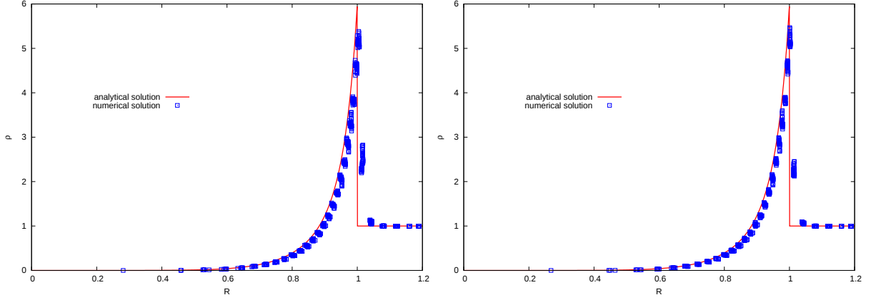
Figure 22: Density in all the cells as a function of cell center radii for the Sedov problem on the polygonal grid at time t = 1 . Area weighted scheme (left) and control volume scheme (right).
