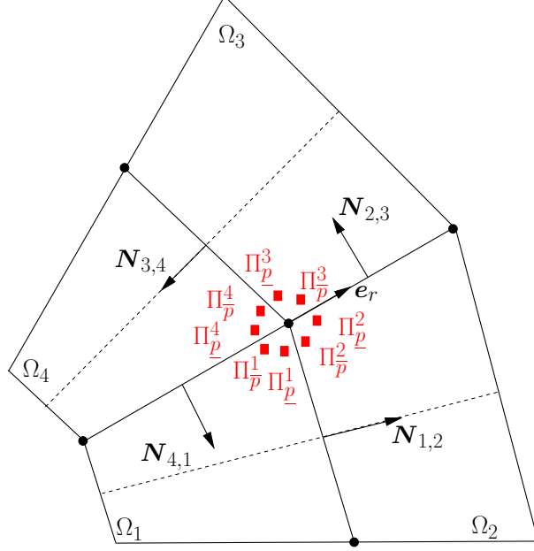
Figure 8: Localization of the multiple nodal pressures around point p .
