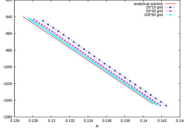
Figure 14: Kidder's isentropic compression. Radial component of the velocity as function of radius versus analytical solution at stopping time t_s = 0.99\tau .
