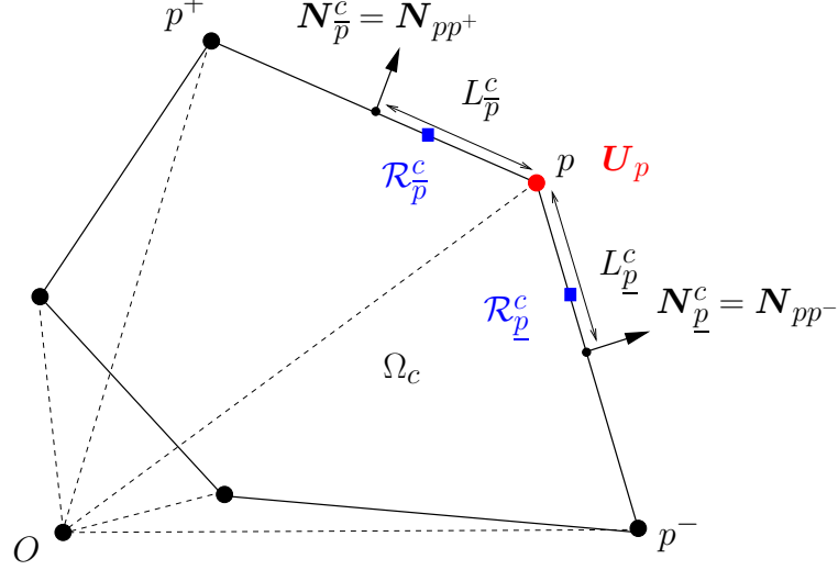
Figure 4: Triangular decomposition of the polygonal cell \Omega_c .
