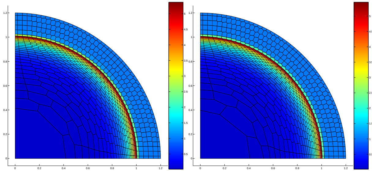
Figure 21: Density map for the Sedov problem on the polygonal grid at time t = 1 . Area weighted scheme (left) and control volume scheme (right).
