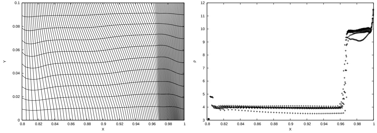
Figure 17: Saltzman piston problem for the area weighted scheme at time t = 0.8 . Grid (left). Density in all the cells as a function of cell-center X coordinate (right).
