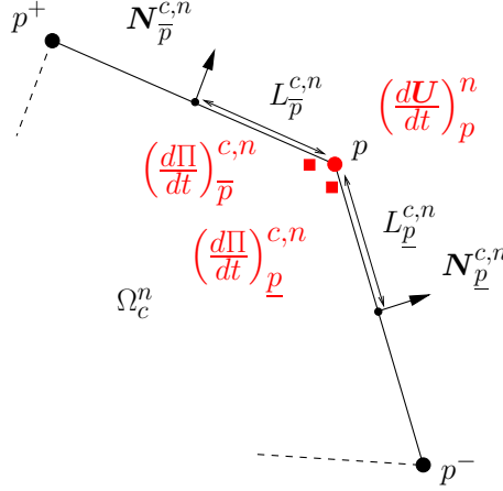
Figure 11: Localization of the time derivatives of the nodal pressures and velocity at point p viewed from cell \Omega_c^n .
