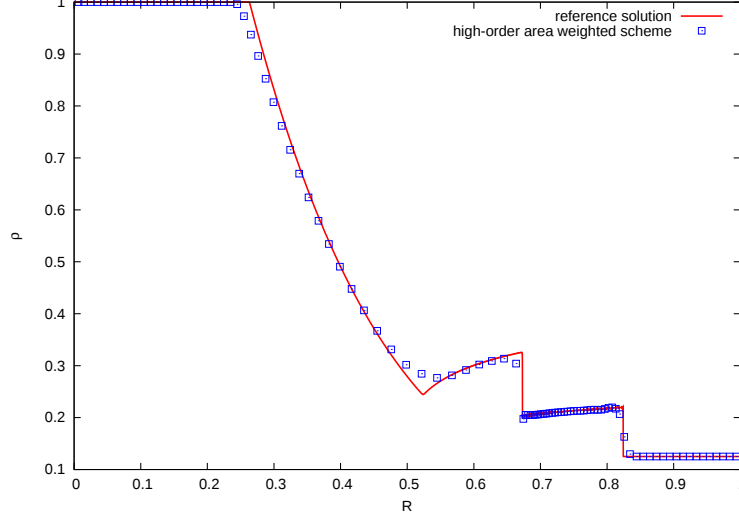
Figure 13: Spherical Sod problem. Density as function of the cell center radius versus reference solution at time t = 0.2 .
