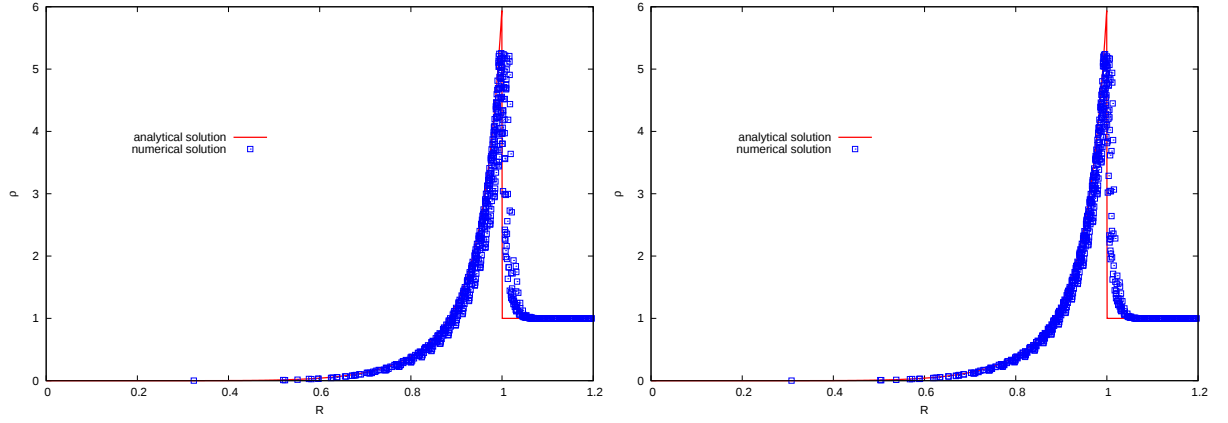
Figure 20: Density in all the cells as a function of cell center radii for the Sedov problem on the Cartesian grid at time t = 1 . Area weighted scheme (left) and control volume scheme (right).
