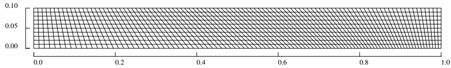
Figure 16: Initial skewed mesh for the Saltzman problem.
