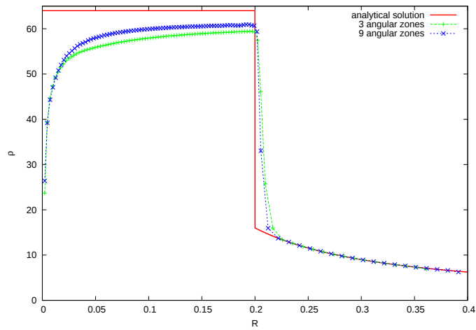
Figure 24: Density as a function of radius for the Noh problem at stopping time t = 0.6 . 3 equal angular zones computation versus 9 equal angular zones computation.
