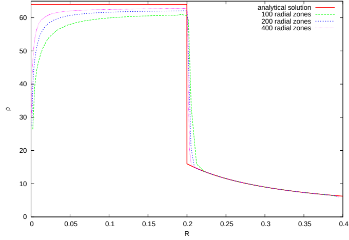
Figure 25: Density as a function of radius for the Noh problem at stopping time t = 0.6 . Convergence analysis.
