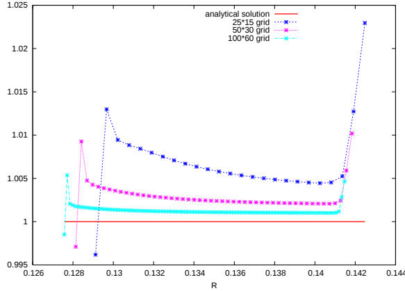
Figure 15: Kidder's isentropic compression. Entropy parameter as a function of radius versus analytical solution at stopping time t_s = 0.99\tau .
