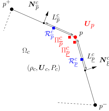
Figure 5: Localization of the nodal pressures given by the half Riemann problems at point p viewed from cell \Omega_c .
