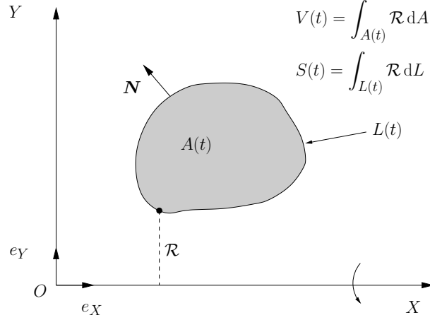
Figure 1: Notations related to the pseudo Cartesian geometry.
