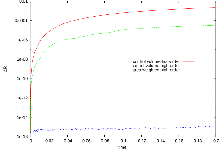
Figure 12: Symmetry preservation indicator as function of time for the spherical Sod problem.
