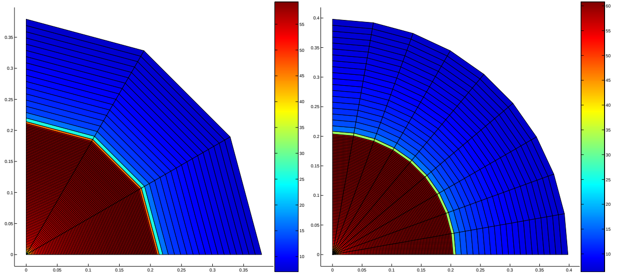
Figure 23: Mesh and density map for the Noh problem at time t = 0.6 . The computations are performed with 100 equal radial zones. The left side computation corresponds to a mesh with 3 equal angular zones whereas the right side one corresponds to a 9 equal angular zones mesh.
