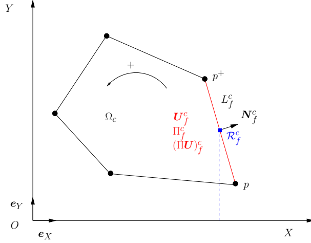
Figure 2: Notations related to the polygonal cell \Omega_c(t) .
