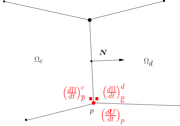
Figure 9: Generalized Riemann problem at point p .
