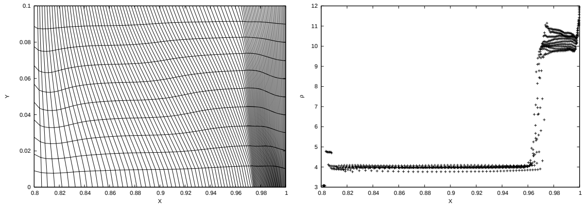
Figure 18: Saltzman piston problem for the control volume scheme at time t = 0.8 . Grid (left). Density in all the cells as a function of cell-center X coordinate (right).
