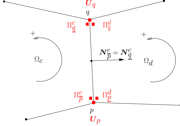
Figure 6: Nodal pressures related to the face [p, q] shared by cells \Omega_c and \Omega_d .
