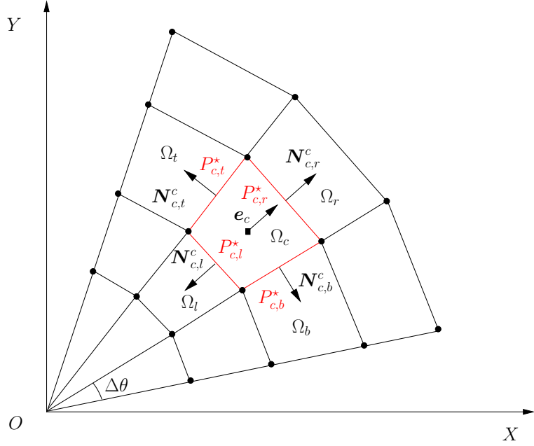
Figure 3: Equal angle polar grid.
