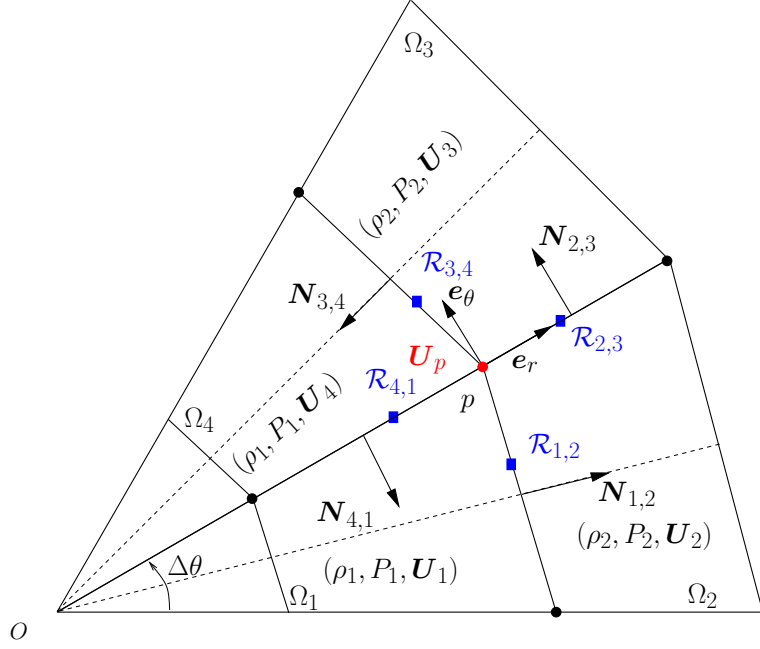
Figure 7: Fragment of an equal angle polar grid and notations for a one-dimensional spherical flow.
