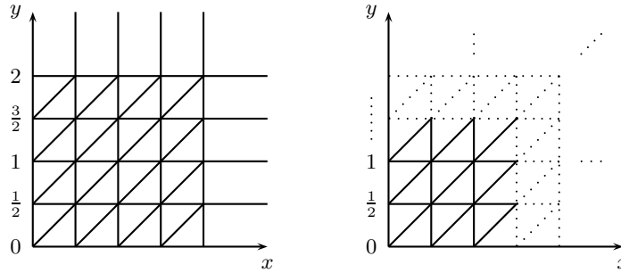
Fig. 3. Partitions of (\mathbb{R}^+)^2 with granularity g = 2 , for K = 2 and K = +\infty
