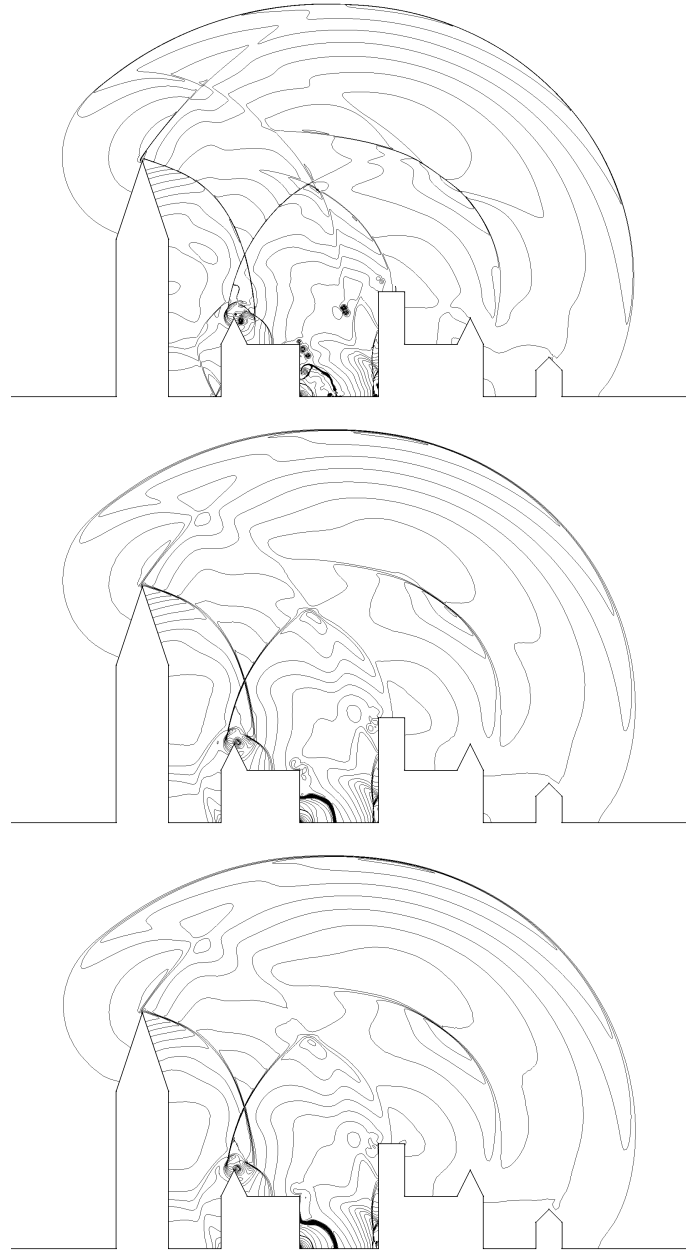
Figure 24: Density isolines from 0.085 to 0.19 with an increment of 2.65 e^{-3} at time t = 0.2 seconds. Top, the reference solution, i.e., \varepsilon = 0.003 and the \mathbf{P}^1 -conservative interpolation. Middle, adapted solution obtained for \varepsilon = 0.006 with the \mathbf{P}^1 -conservative interpolation. Bottom, adapted solution obtained for \varepsilon = 0.006 with the \mathbf{P}^1 -interpolation.
