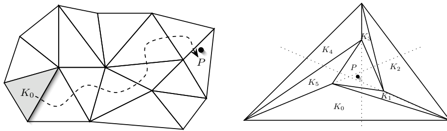
Figure 3: Left, a possible path to locate the vertex P of the new mesh starting from the triangle K_0 of the background mesh. Right, cyclic path leading us to an already checked element. Starting from K_0 , triangles K_1 , K_2 , K_3 , K_4 and K_5 are visited bringing us back to K_0 .
