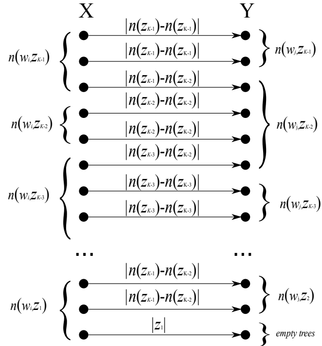
Figure 22: Bipartite Matching Problem in the general case
