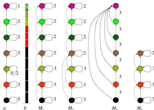
Figure 8: Differentiation graphs used for the definition of theoretical plants. a) The differentiation graph of a non-branching plant structure. b) The resulting axis structure, where component colors correspond to the differentiation graph states in which these components were created. The numbers attached to each loop indicate the number of steps a meristem stays in the corresponding state. Right: The differentiation graphs of models M_1 , M_2 , M_3 and M_0 . Solid arrows correspond to possible transitions of the apical meristem states. Dashed arrows correspond to possible transitions from the apical meristem state to the axillary meristem states.
