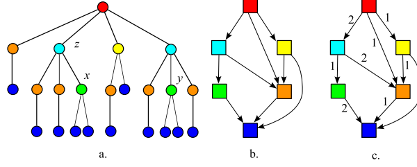
Figure 1: a. A rooted tree T . Isomorphic nodes are colored identically: T[x] \equiv T[y] and z \preceq x then T[y] \subseteq T[z] . b. Quotient graph \mathcal{Q}(T) associated with T : vertices of this graph are equivalence classes colored according to the color of the class of isomorphic vertices they represent in T . c. Reduction graph of T corresponding to \mathcal{Q}(T) whose edges are labeled with the signature distribution function n .
