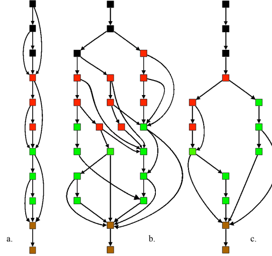
Figure 12: DAGs corresponding to the reductions of tree individuals in the families a. T_0 , b. T_{0,4} and c. T_{0,8} .
