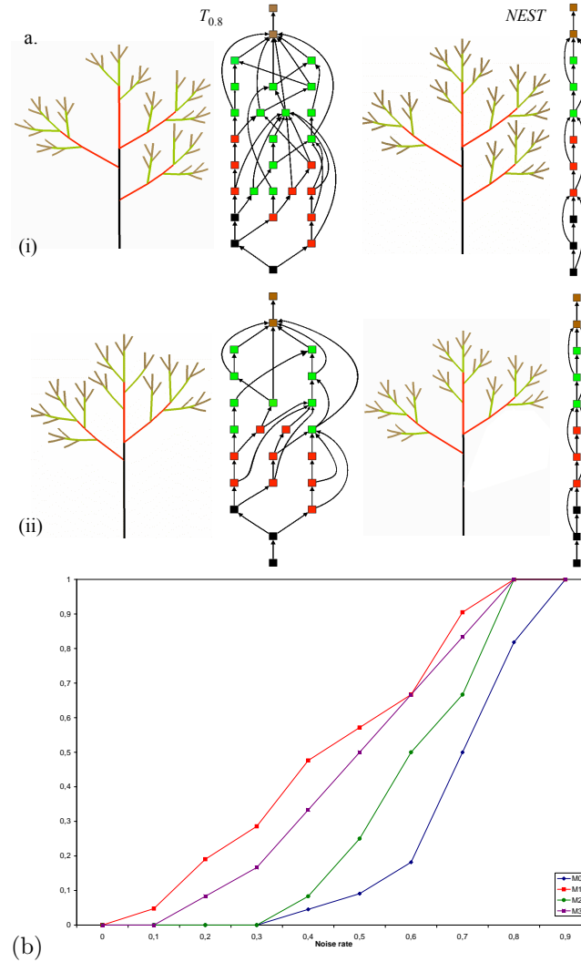
Figure 17: a. Two random versions of T_{0.8} such that (i) the NEST is isomorphic to the template or (ii) not. b. Cumulated percentage of plants from the different families having a NEST isomorphic to their template plant as a function of noise.
