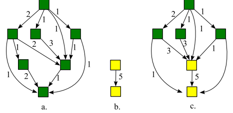
Figure 5: a. a DAG G b. a linear DAG L such that h(L) \leq h(G) . c. DAG G \langle L \rangle corresponding to the DAG G partially linearized by L .
