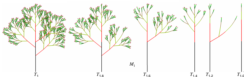
Figure 9: Deterministic model T_1 and 5 of its random versions from the plant samples T_{1,8} , T_{1,6} , T_{1,4} , T_{1,2} , T_{1,0}
