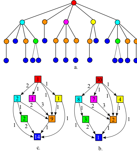
Figure 2: a. A tree T whose vertices are colored according to their signature. b. Corresponding reduction graph showing the value with n(I) on each vertex. c. Reduction graph where vertices are valuated with m(I) . Both quantities are computed recursively.
