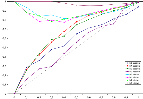
Figure 13: Average vertex absolute and relative compression factors ( \rho_v(T) and \rho'_v(T) ) of the trees in the \mathcal{T}_i families, i = 0, 1, 2, 3 (standard deviations are not shown here). Curves passing through the point (0,0) correspond to the absolute coefficients.
