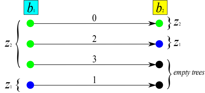
Figure 21: Bipartite Matching problem associated with Fig. 7c.
