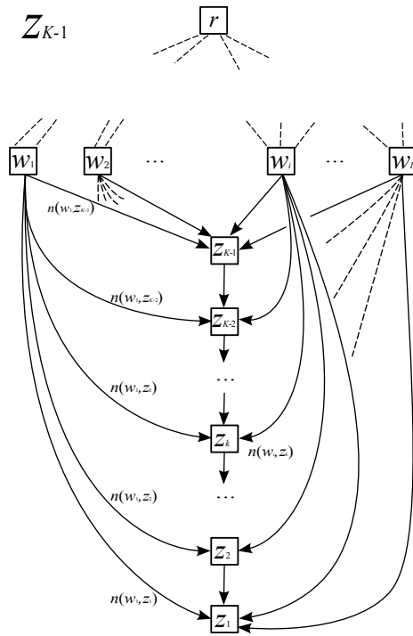
Figure 6: DAG Z_{K-1} . The minimization D(Z_{K-1}, H) for H \in \mathcal{S}_K^+(Z_{K-1}) consists of merging all the vertices at level K in a minimal way to obtain a new DAG in \mathcal{S}_K^+(G) , i.e. linearized up to height K
