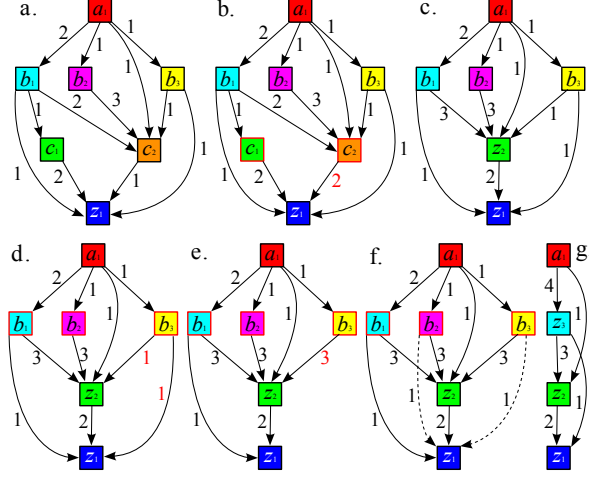
Figure 7: The seven steps of the algorithm needed to find the nearest linear DAG of the DAG introduced in Fig. 2
