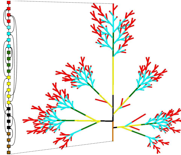
Figure 20: a. An element T^* of NEST(T) b. Backward projection of the differentiation states inferred from T^* onto the initial tree structure of the panicle (see text for color interpretation).
