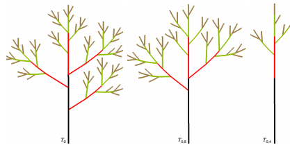
Figure 10: The \mathcal{T}_0 family: (a) template plant T_0 and random trees from (b) \mathcal{T}_{0,8} and (c) T_{0,4} .
