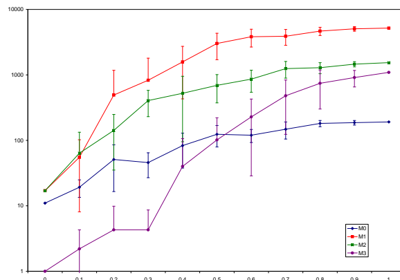
Figure 15: Average number of vertices in NEST(T) for trees of the different families as a function of the branching probability.
