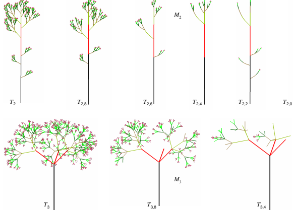
Figure 11: Top row: template plant T_2 and trees in \mathcal{T}_{2,i} for i = 8, 6, 4, 2, 0 . Bottom row: T_3 and 2 of its random versions from \mathcal{T}_{3,8} , \mathcal{T}_{3,4} .
