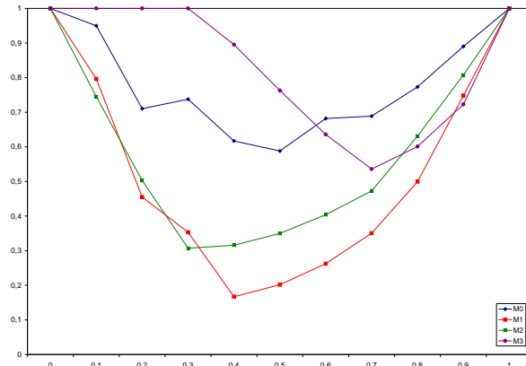
Figure 16: Average degree of self-nestedness depending on the branching probability.
