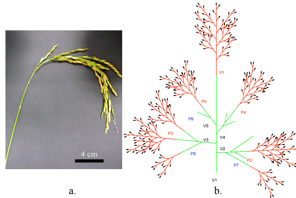
Figure 18: a) photo of a rice panicle (courtesy of Y. Caraglio). b) corresponding topological structure (reconstructed with the AMAPmod/VPlants open software [62]).
