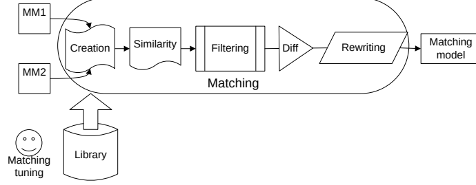
Figure 8: Matching Strategy Overview
