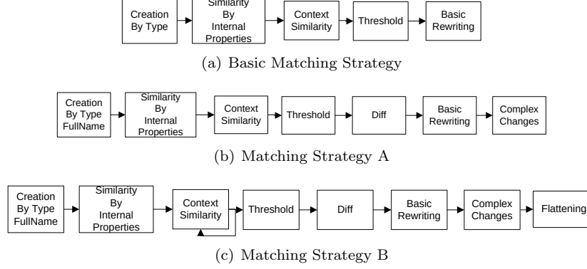
Figure 9: Matching Strategies
