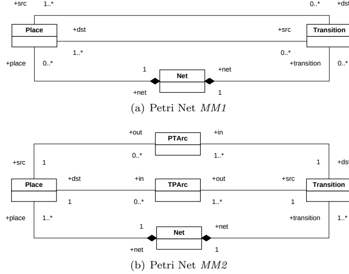
Figure 2: Petri Net metamodells
