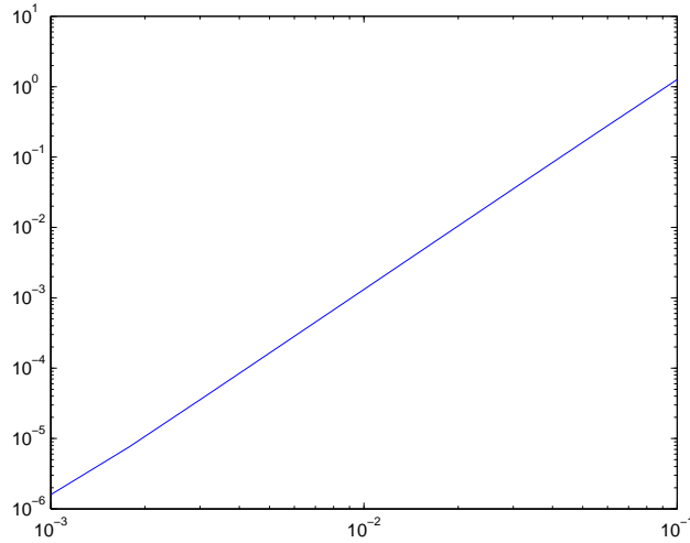
Figure 6.10: \sum_{\pm} \|\widehat{u}_\pm^{\varepsilon, app} - \widehat{u}_\pm^\varepsilon\|_{H^1(\widehat{\Omega}_\pm^\delta)} as function of \varepsilon (logscale)
