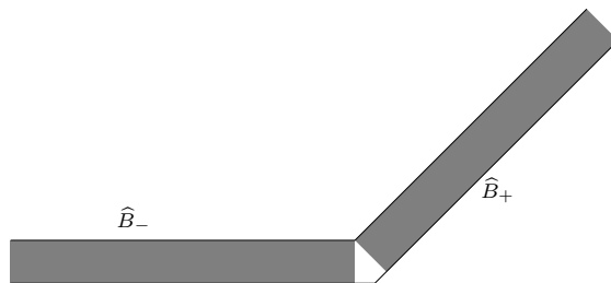
Figure 2.3: The subdomains \widehat{B}_\pm
