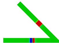
Figure 6.7: \alpha = \frac{3\pi}{8}
