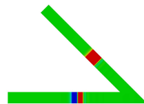
Figure 6.7: \alpha = \frac{3\pi}{8}
