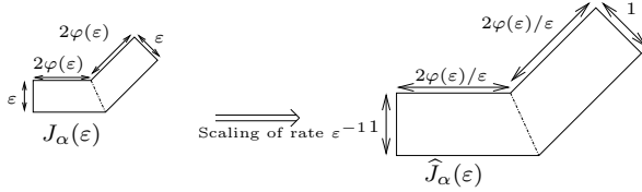
Figure 2.1: The near-field zone
