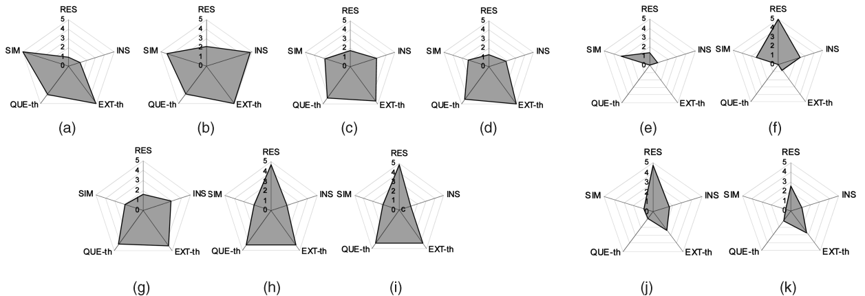
Fig. 11. SP-x, SPJ-x and SPJG-x DBMS alternatives. (a) SP-FS SF = 1. (b) SP-DS SF = 1. (c) SP-RS SF = 1. (d) SP-RIS SF = 1. (e) SPJ-RS SF = 1. (f) SPJ-RS SF = 25. (g) SPJ-RS SF = 40. (h) SPJG-FS SF = 25. (i) SPJG-DS SF = 25. (j) SPJG-RS SF = 25. (k) SPJG-RIS SF = 25.
