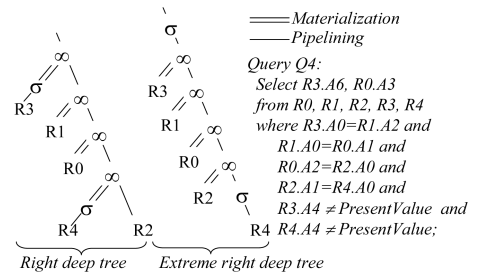
Fig. 5. Extreme right deep tree example (Query Q4).
