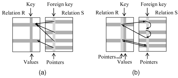
Fig. 4. Storage models for foreign key attributes. (a) DS. (b) RS.
