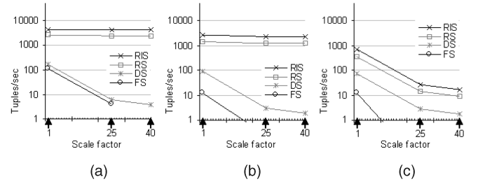
Fig. 10. SPJG alternatives—throughputs for extractions. (a) SPG query. (b) SPJG query. (c) SPJG n query.
