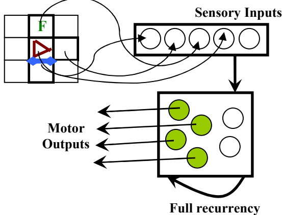
Figure 1. Schematic view of neural "brain" of the animat. It senses only its immediate environment, with 4 input giving information on presence of something (food, poison or wall on current and 3 adjacent cells in front/left/right, and a last input giving a local smell (random in case nothing is present). The "brain" is a fully recurrent network with N \geq 4 neurons, including the 4 motor output neurons.
