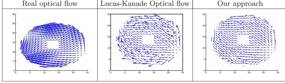
Fig. 4. Optical flow with translation tx = 2cm ty = 1cm
