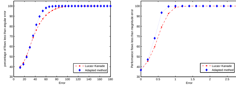
Fig. 9. Relative performance of the two algorithms with sequence :translation tx = 4cm ty = 2cm . Left: percentage on angle error. Right: magnitude of difference performance
