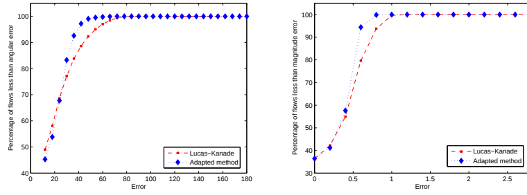
Fig. 10. Relative performance of the two algorithms with sequence :rotation around Z-axis of 1. Left: percentage on angle error. Right: magnitude of difference performance
