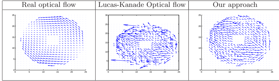
Fig. 5. Optical flow with translation tx = 4cm ty = 2cm
