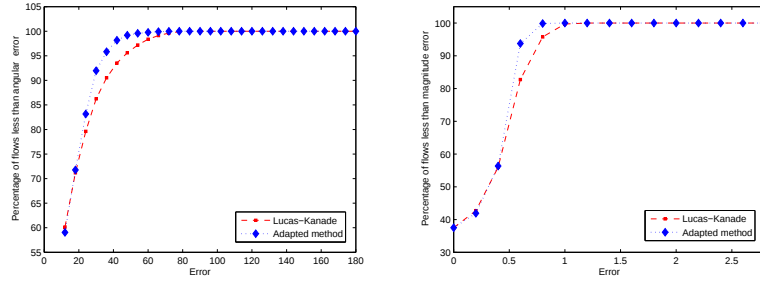
Fig. 8. Relative performance of the two algorithms with sequence :translation tx = 2cm ty = 1cm . Left: percentage on angle error. Right: magnitude of difference performance.
