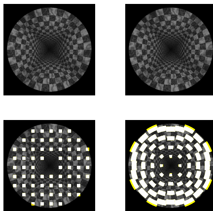
Fig. 3. Top: Example of synthetic images. Bottom left: The fixed and classical neighborhood , bottom right: Adapted neighborhood
