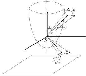
Fig. 2. Adapted neighborhood for catadioptric images
