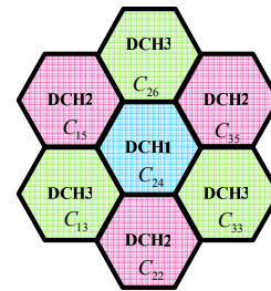
b. Control channel allocation inside G'_{24} .
