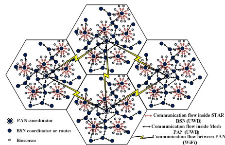
Fig.1 WHSN architecture
