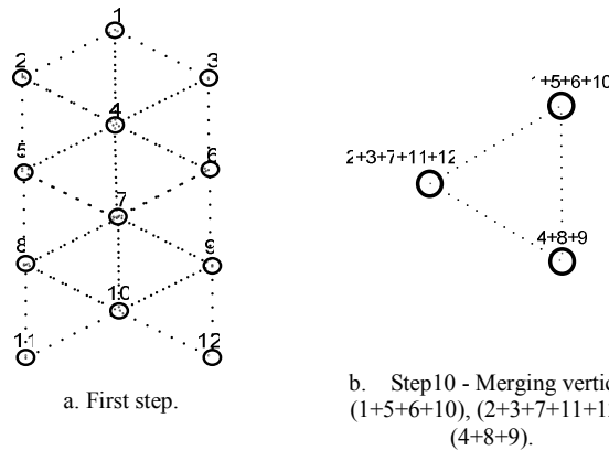
Fig.11 Logical data communication channel allocation graph
