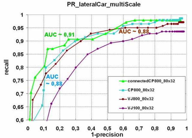
Fig. 6: Precision-recall curves for adaBoost lateral car detectors obtained with connected-control-points features (upper green curve), standard control-points (cyan curve), and ViolaJones Haar-like features (maroon)
