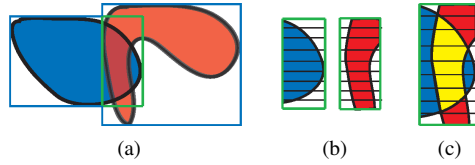
Figure 3: The LDI process. (a): AABBB computations, (b): Rasterization of each object, (c): Volume intersection.
