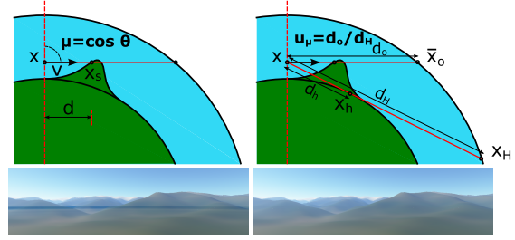
Figure 3: Viewing angle parameter. Left: using \mu gives artifacts. Right: using u_\mu = d_o / d_h or d_o / d_H solves the problem (using 128 values for \mu or u_\mu in the precomputed sky radiance table \mathbb{S} ).
