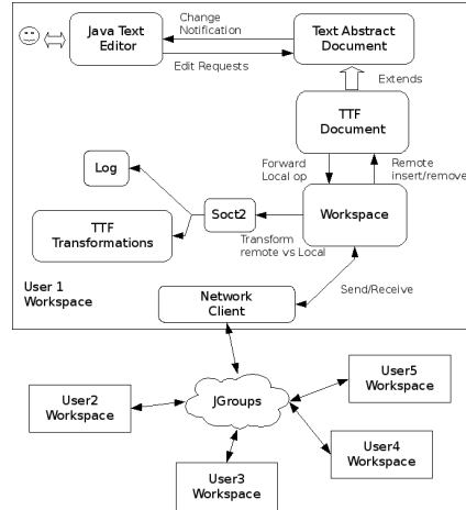
Figure 12: Graveyard architecture
