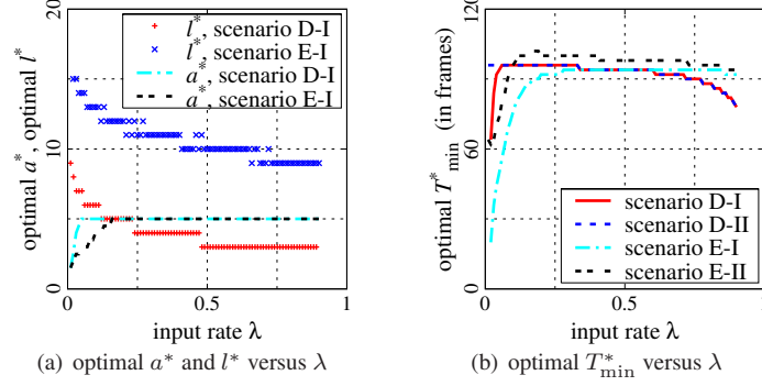
Figure 10: Optimal values of the protocol parameters from programs \mathcal{P}_1 – \mathcal{P}_3 .
