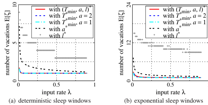
Figure 11: Expected number of vacations E[\xi] versus \lambda when the protocol parameters are optimally set.
