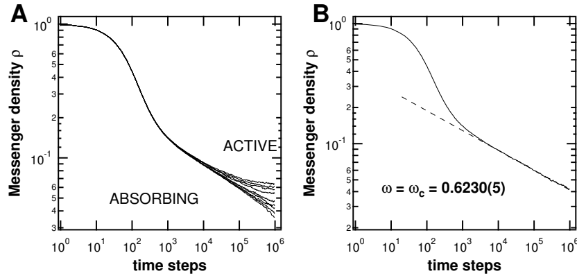
Figure 4: Dynamics of the messenger density \rho(t) close to the boundary between active and absorbing phases. (A) Each curve corresponds to a different value of \omega , i.e., from bottom to top, \omega = 0.6220, 0.6225, 0.6230, 0.6235, 0.6240, 0.6260, 0.6270, 0.6280 and 0.6290 . (B) Time-variation of \rho when \omega is set to its estimated critical value \omega = \omega_c = 0.6230(5) . (The number between parentheses denotes the estimated incertitude on the last digit). The dashed curve indicates a power-law decay with exponent -0.165 . Parameters were \lambda = 0.0150 and other parameters from the standard set (c.f. 2.e).
