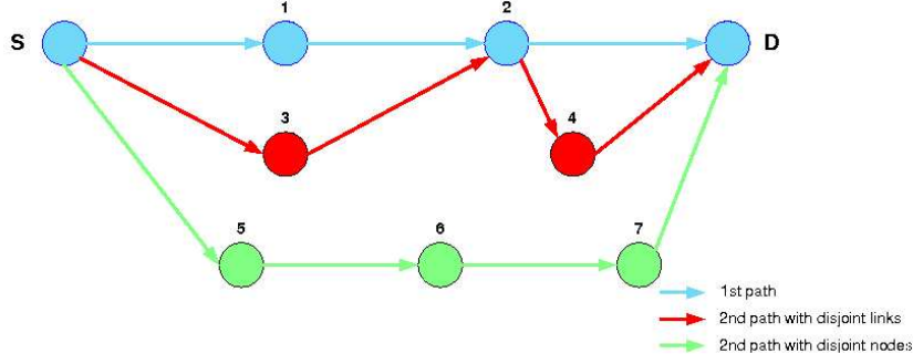
Figure 6: Multipath routing
