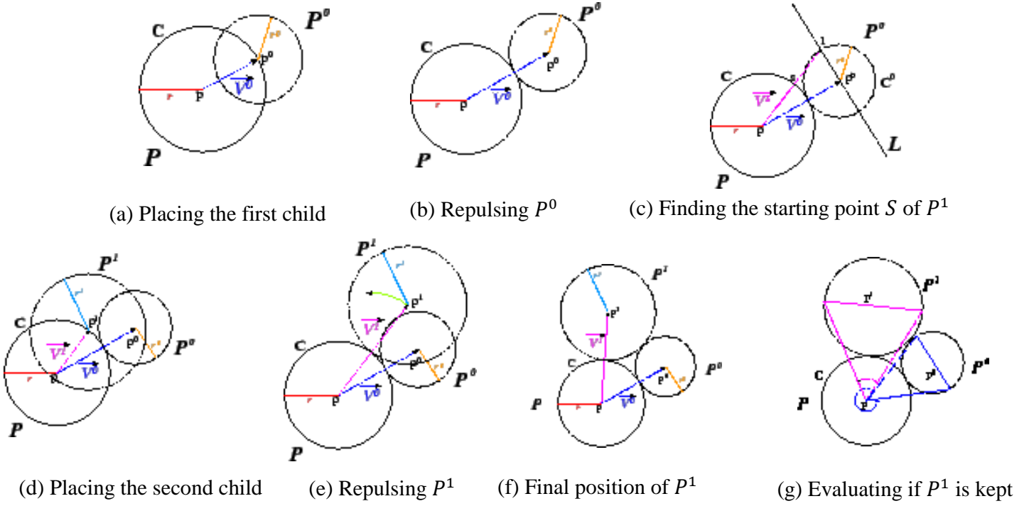
Figure 7 Generation of the first two children of P : first, P^0 is placed anywhere on C (a) and then is repulsed in the direction \vec{V}^0 until it reaches its final position (b). Thus we find the starting point S of P^1 thanks to the point I (c). The second child P^1 is then created (d) and repulsed in direction \vec{V}^1 (e). This time P^1 intersects P^0 so P^1 is repulsed on the circle C (f). Finally, when its final position is reached, we test its projection on C (thanks to \varphi ) in order to determine if P^1 is added to the set or not.
