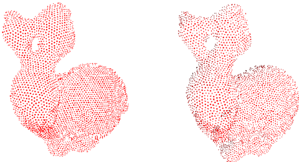
Figure 9 The bunny sampled with around 10,000 particles using (left) our method and (right) the Witkin and Heckbert one.
