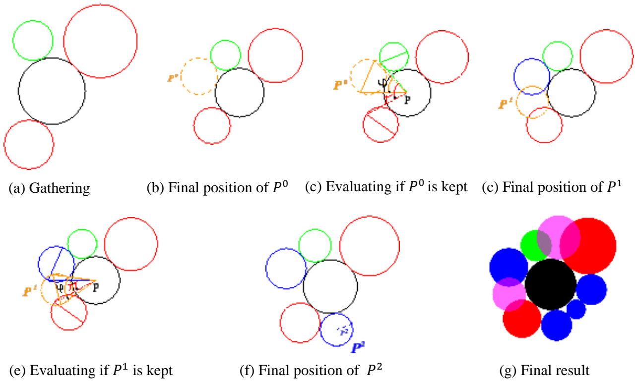
Figure 8 Generation of the children of P (the black particle) with respect to existing particles (red particles). Its father is green while blue particles are generated particles added to the set. Finally, the orange particle is the the current generated particle. First we gather the neighboring particles of P (a). We then find the final position of the current generated particle (b-d-f). We estimate its projection on C (thanks to the angle \varphi ) and compare it with the free circumference of C given by the angle \tau (c-e) in order to determine if it is added to the set or not. The final result is that some generated particles have been added to the set (blue particles) while others have not (transparent violet particles) (g).
