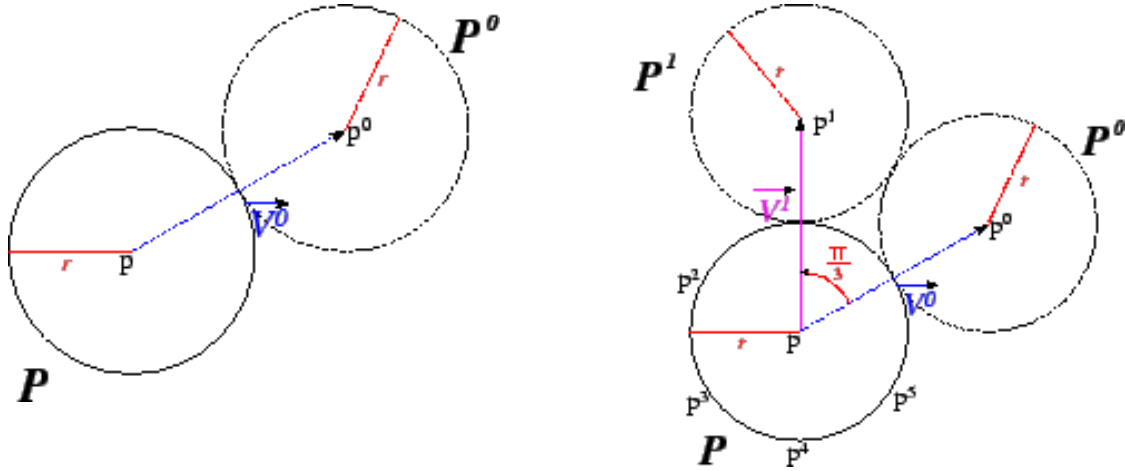
Figure 3 Generation of particles in the 2D tangent plane. (left) The first particle is generated using an arbitrary direction. (right) The second child is placed at an angle of \pi/3 .
