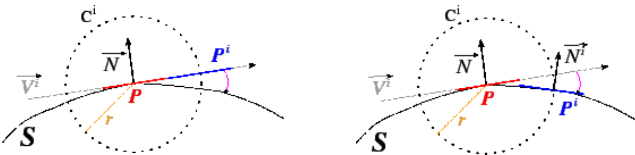
Figure 4 Re-projecting a particle on the surface. (left) Initial position of the child P^i . (right) P^i is reprojected according to circle C^i .
