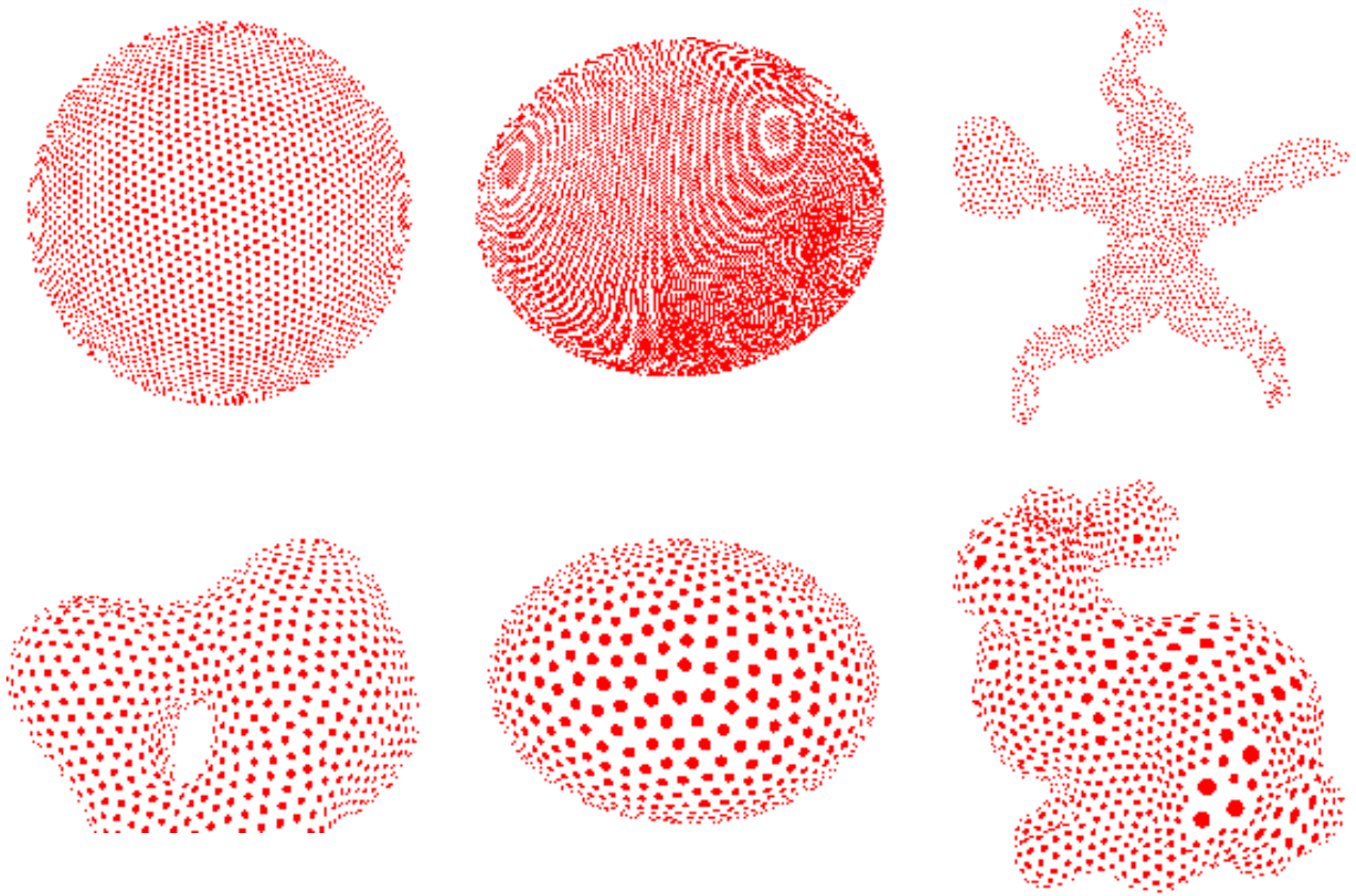
Figure 12 Examples of our two sampling techniques.
