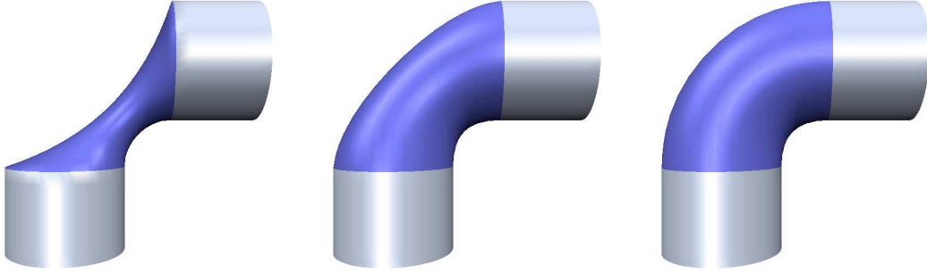
Figure 7.6: The order k of the energy functional and of the corresponding Euler-Lagrange PDE \Delta_S^k \mathbf{x} = 0 defines the stiffness of the surface in the support region and the maximum smoothness C^{k-1} of the boundary conditions. From left to right: membrane surface ( k = 1 ), thin-plate surface ( k = 2 ), minimum variation surface ( k = 3 ).
