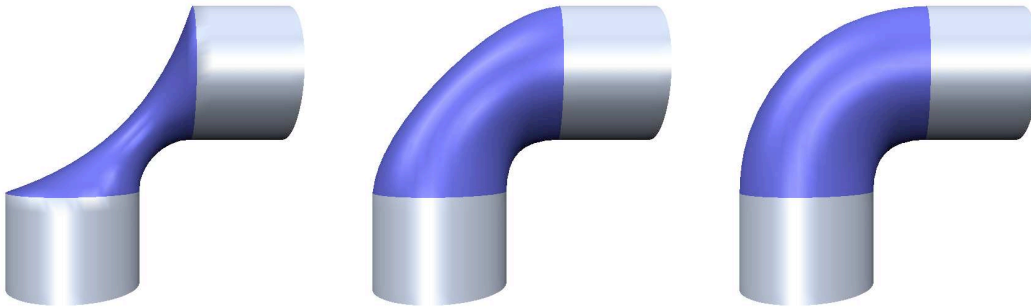
Figure 2.1: This figure shows three examples of fair surfaces, which define a blend between two cylinders. On the left there is a membrane surface which minimizes the surface area. In the center, a thin-plate surface which minimizes curvature. On the right there is a surface which minimizes the variation of mean curvature.
