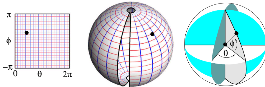
Figure 8.5: Spherical coordinates
