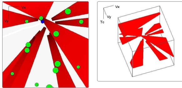
Fig. 1. NLVO examples In \mathcal{V} (left) the green disks represent the obstacles, the blue one is the robot, and the red shapes (one by obstacle) constitute the NLVO . The expression of the NLVO in \mathcal{V} \times \mathcal{T} (right) gives an extra information on the time to collision associated with each velocity.
