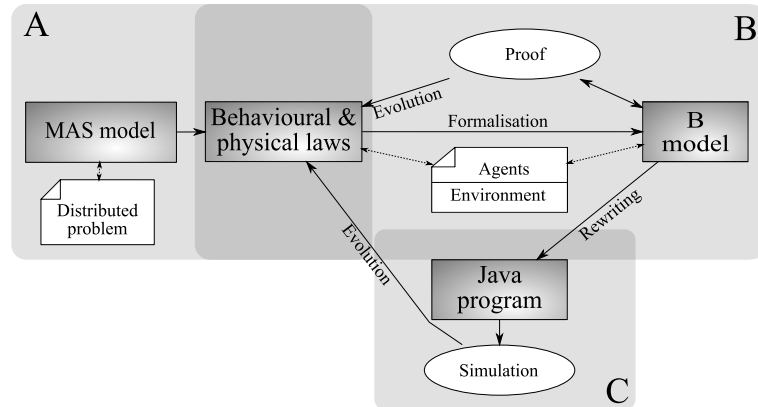
Figure 12: A general development processus
