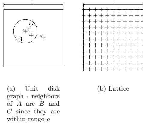
Figure 1: Network Models
