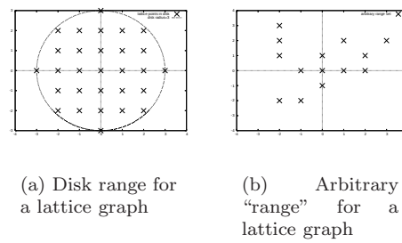
Figure 2: Examples of range for lattices
