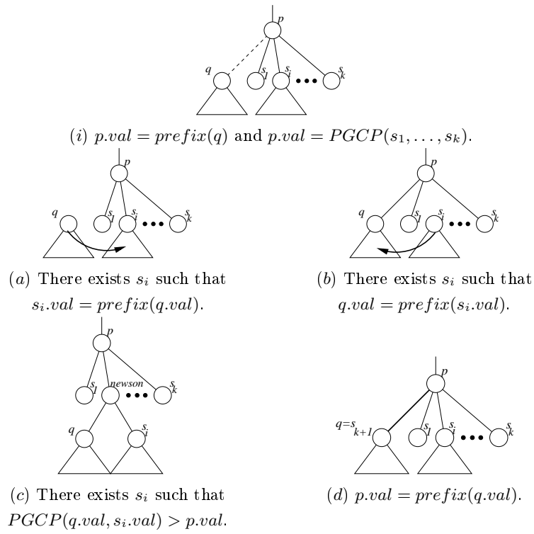
Figure 1: A false root q is linked to a node p such that p.val = prefix(q.val) .
