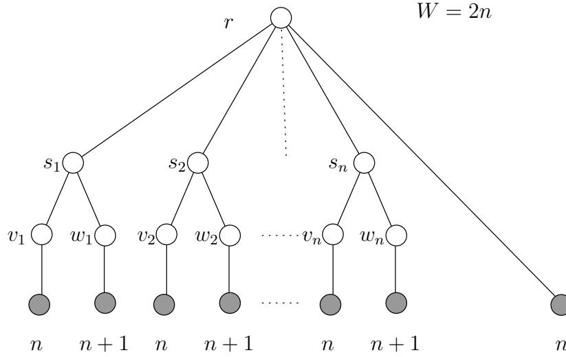
Figure 3: Multiple versus Upwards , homogeneous platforms.
